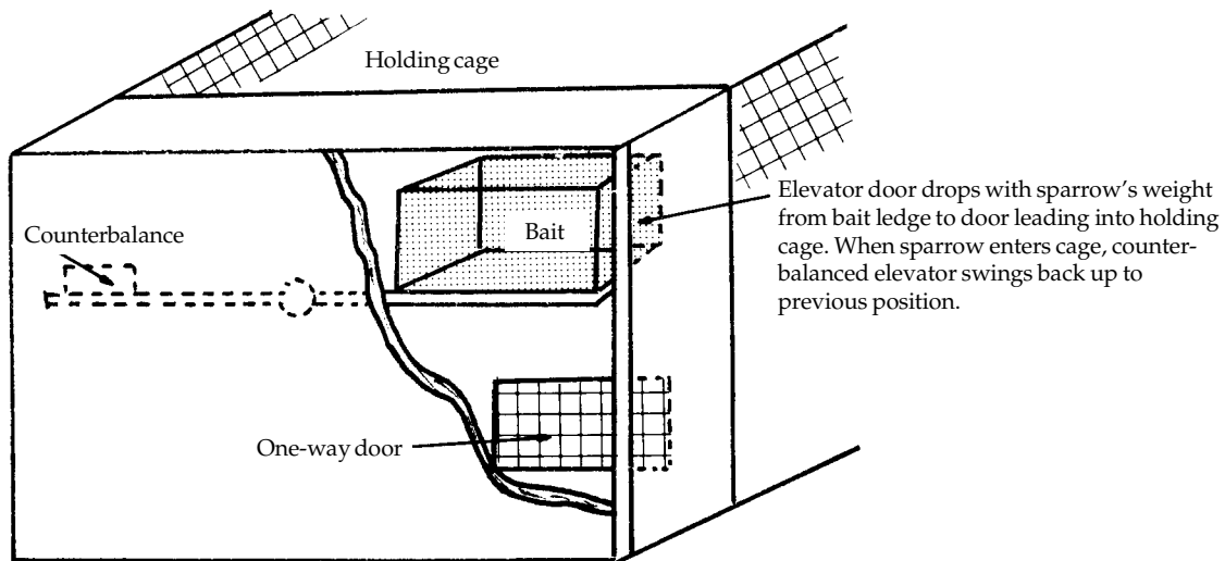
Havahart elevator trap
